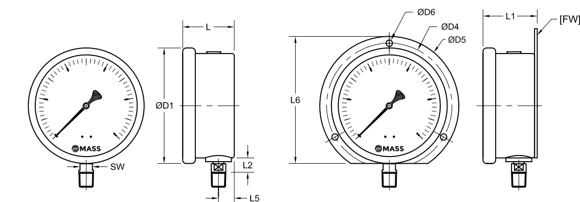
Lower Connection Direct Mounting
